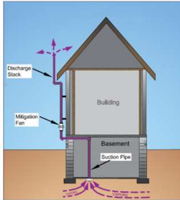
Basement Mitigation System
